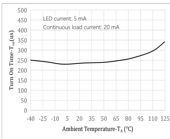
Fig.5 Turn On Time vs. Ambient Temperature Characteristics
