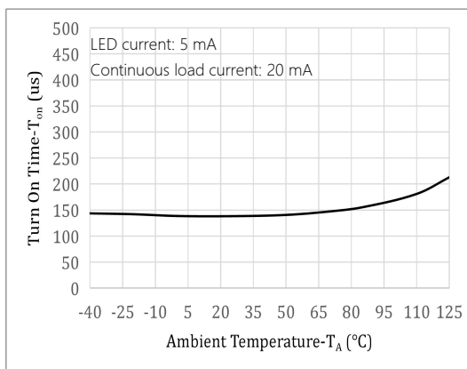
Fig.7 Turn On Time vs. Ambient Temperature
