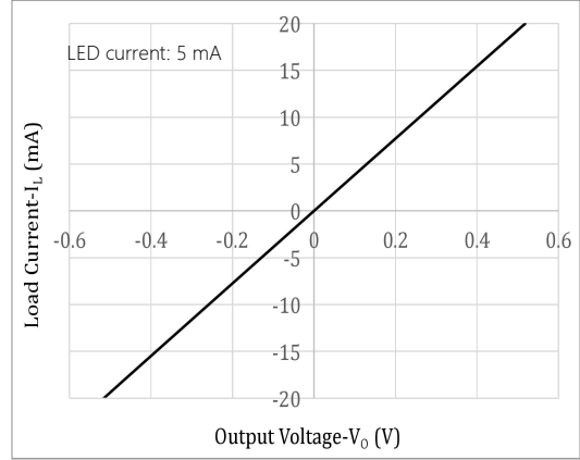
Fig.2 Load Current vs. Output Voltage Characteristics
