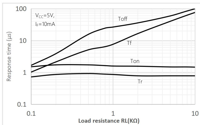
Fig.7 Response Time vs. Load Resistance
