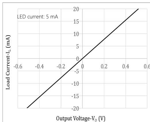
Fig.2 Load Current vs. Output Voltage Characteristics
