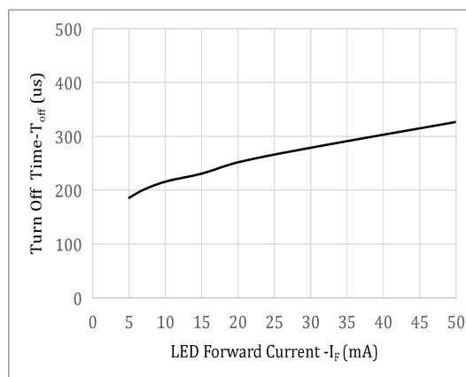
Fig.12 Turn On/Off Time
