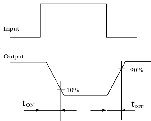
Fig.11 Turn On/Off Time
