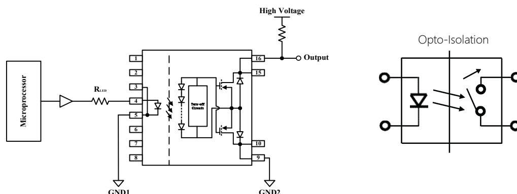
Fig.12 Typical Application Circuit
