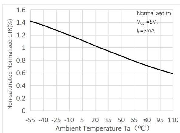
Fig.5 Non-saturated Normalized CTR vs. Ambient Temperature
