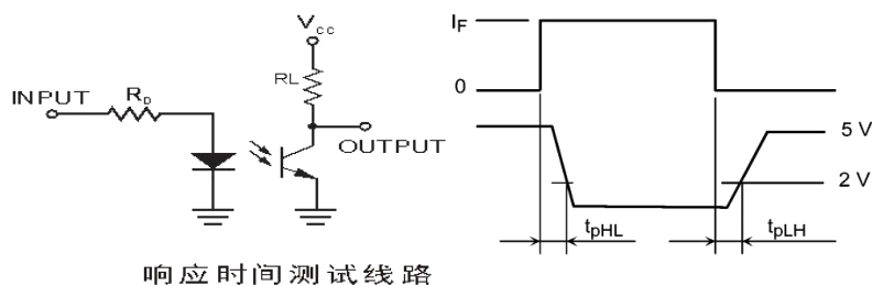
Fig.10 Propagation delay Time Test Circuit & Wave forms
