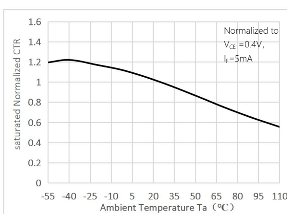
Fig.6 Saturated Normalized CTR vs. Ambient Temperature
