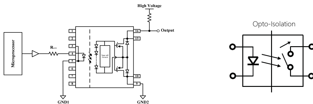
Fig.13 Typical Application Circuit
